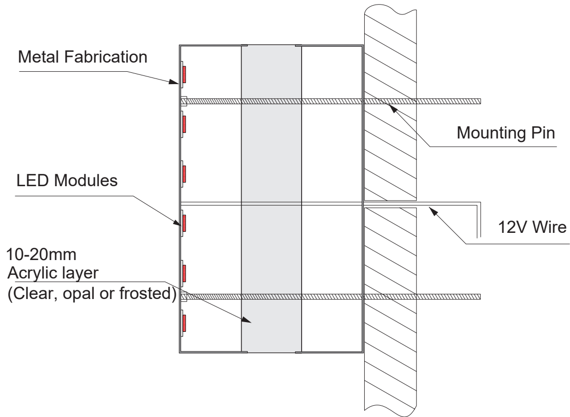
Side View Flush Mount
